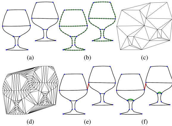
Figure 4: Constructing the Graph: (a) An initial graph is inferred according to the edges of the image. (b) Additional vertices are created at fixed intervals within each line segment. (c) A Delaunay triangulation T(V) of the original vertices is calculated. (d) A second triangulation T(V') is calculated from the new set of vertices. (e) Auxiliary edges (in red) are inserted in order to merge the disconnected graph components, based on the edges of both triangulations. (f) Duplicate edges (in green) are created in order to Semi-Eulerize the graph.
