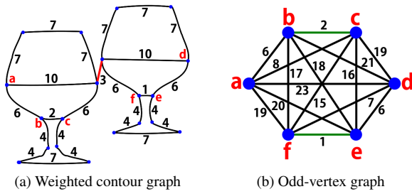
Figure 5: Semi-Eulerization steps: (a) A graph with several odd-degree vertices (labeled in red). (b) A complete graph G_o is built upon the odd-degree vertices of the input graph. Vertex matchings (in green) are chosen in a greedy manner in our approach.
