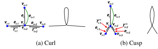
Figure 7: Curl or cusp?: (a) A sequence of line segments is converted into a curl feature. (b) A sequence of line segments is converted into a cusp feature.
