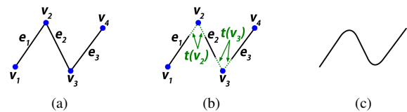
Figure 6: Trimming and reconnecting: (a) Original segments in the Eulerian path. (b) Line segments are trimmed by a distance t(v_i) . (c) Connecting curves are traced between the endpoints of subsequent line segments in the path.
